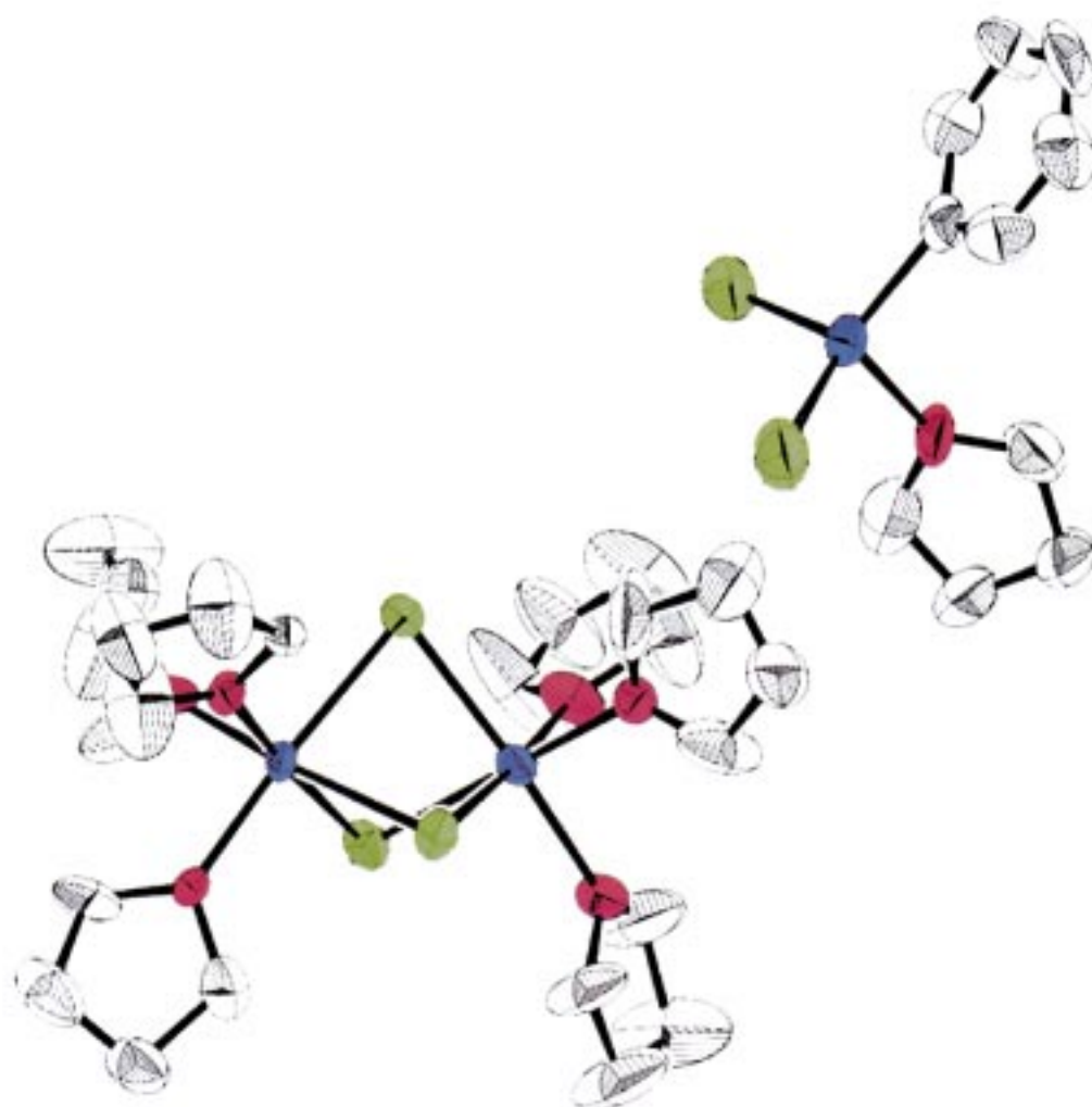
ORTEP drawing of [2\text{Mg}_2(\mu\text{-Cl}_3)(\text{THF})_6]^+\bullet\text{PhMgCl}_2(\text{THF})^- , Mg: Blue, Cl: Green and O: Red.
