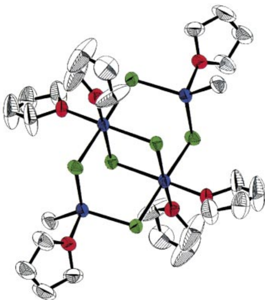
ORTEP drawing of Me 2 Mg 4 Cl 6 (THF) 6 , Mg: Blue, Cl: Green and O: Red.
