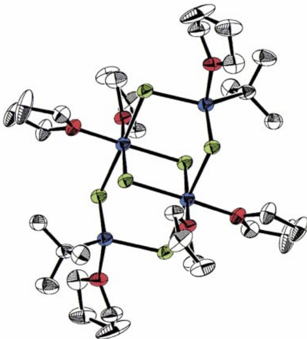
ORTEP drawing of t\text{Bu}_2\text{Mg}_4\text{Cl}_6(\text{THF})_6 .
